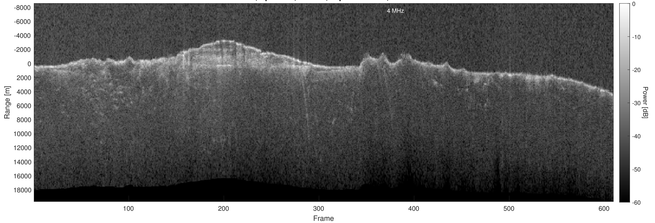
Orbit 6448, Optimized, Window, Depth-Corrected, Channel 2
