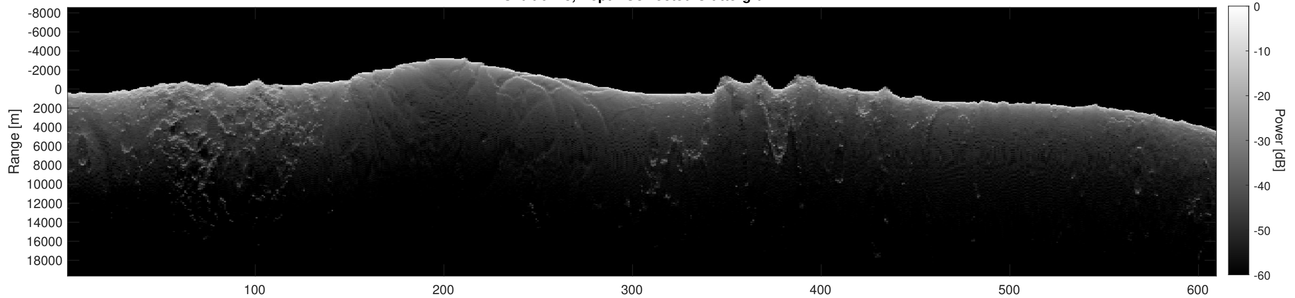
Orbit 6448, Depth-Corrected Cluttergram
