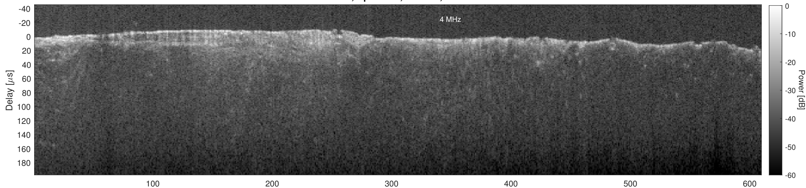
Orbit 6449, Cluttergram
