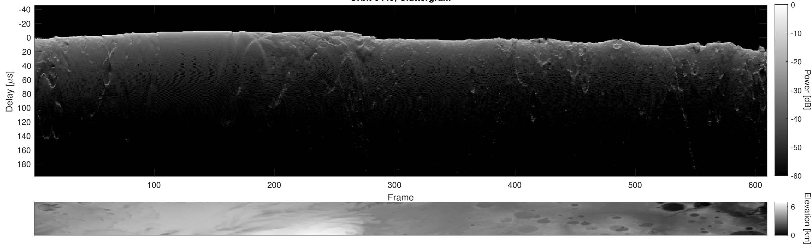
Orbit 6449, Cluttergram
