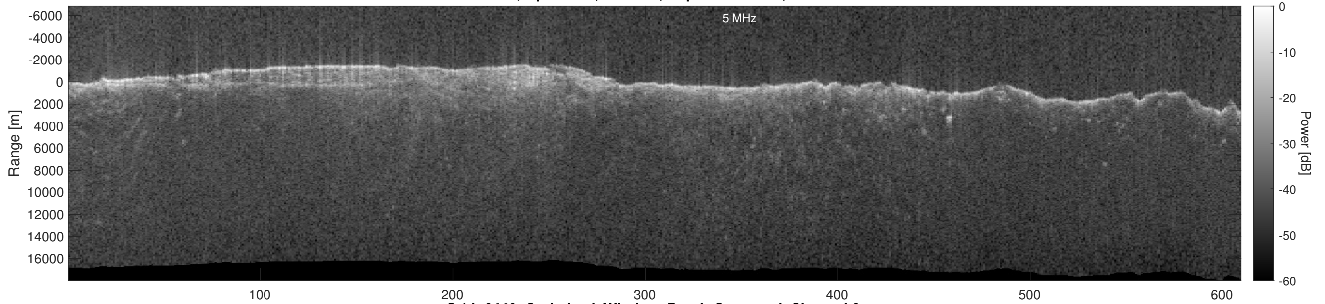
Orbit 6449, Optimized, Window, Depth-Corrected, Channel 2
