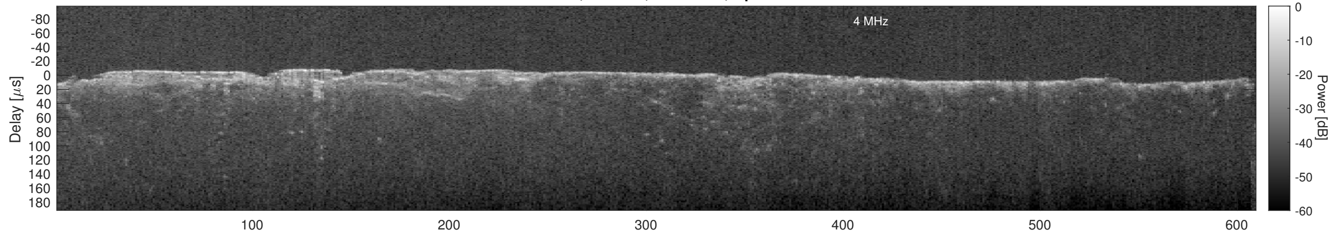
Orbit 6453, Cluttergram
