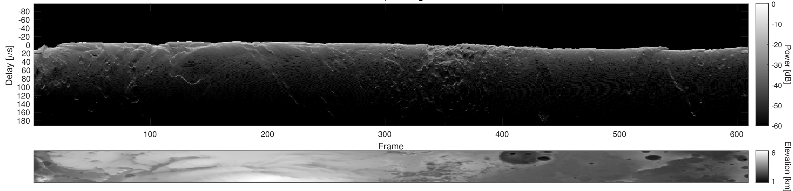
Orbit 6453, Cluttergram
