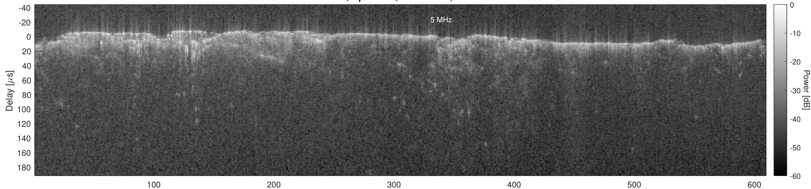
Orbit 6453, Optimized, No Window, Channel 2
