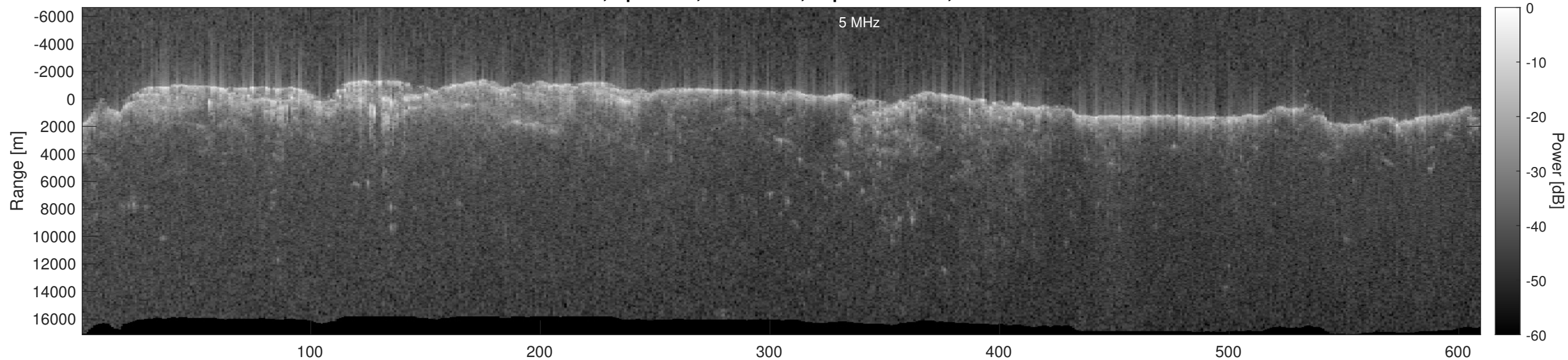
Orbit 6453, Optimized, No Window, Depth-Corrected, Channel 2
