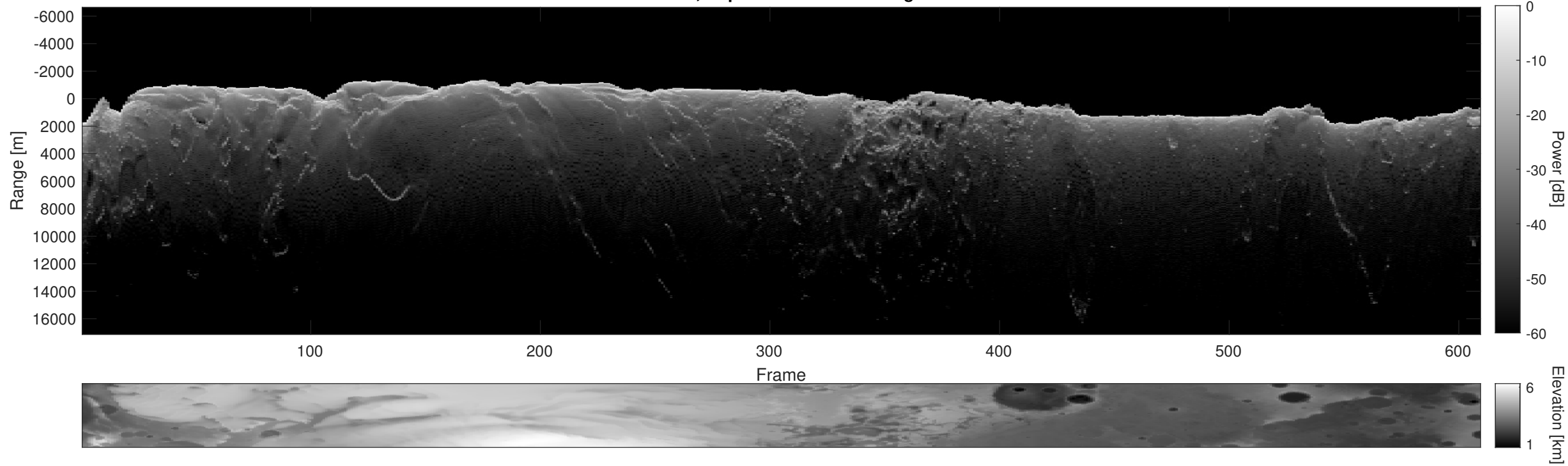
Orbit 6453, Depth-Corrected Cluttergram
