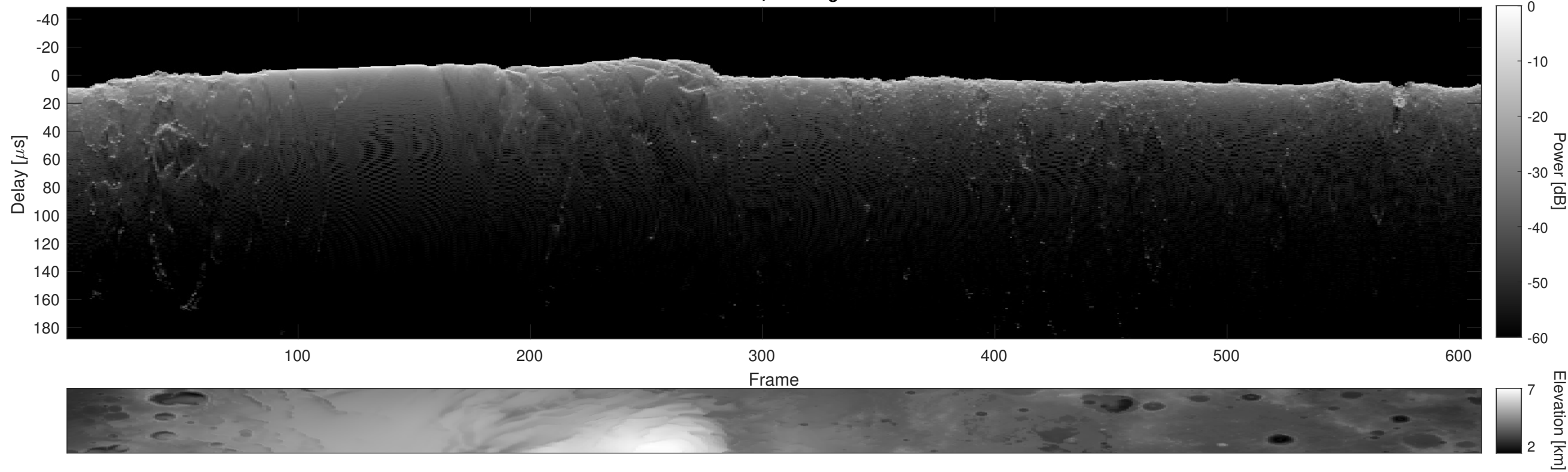
Orbit 6456, Cluttergram
