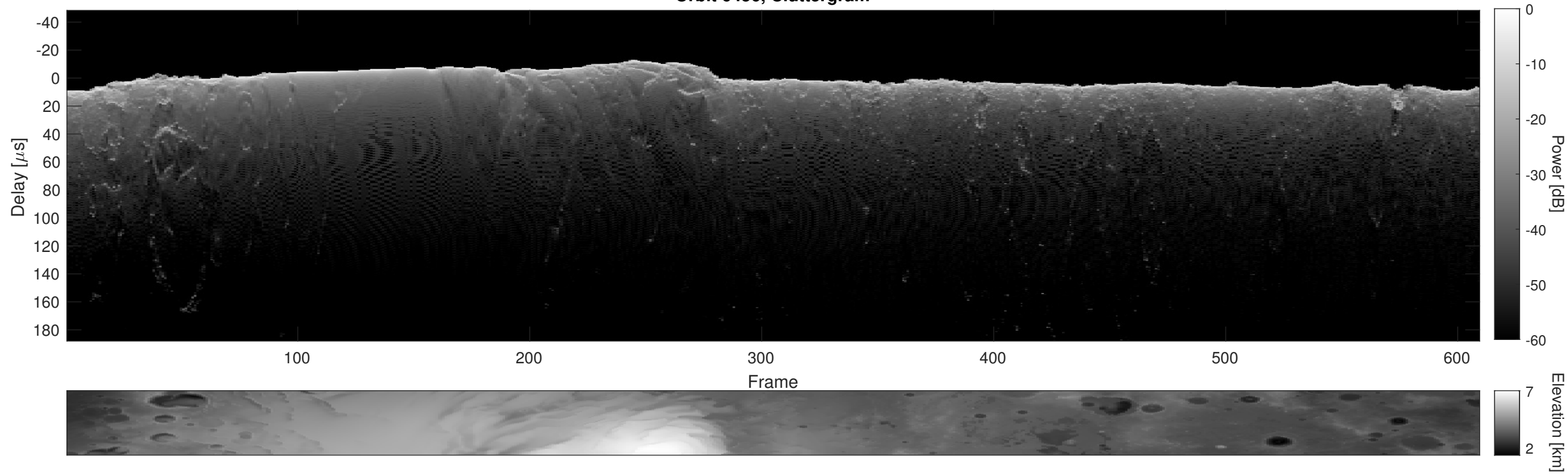
Orbit 6456, Cluttergram
