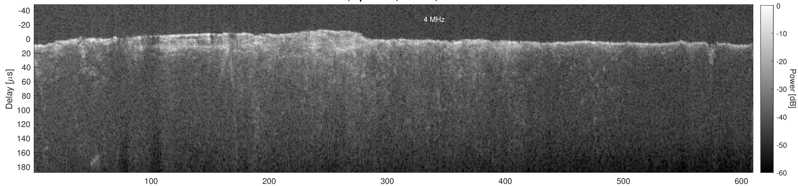
Orbit 6456, Cluttergram
