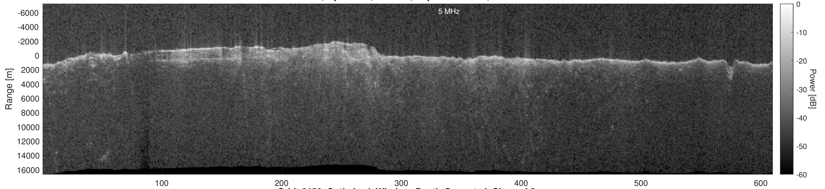
Orbit 6456, Optimized, Window, Depth-Corrected, Channel 2
