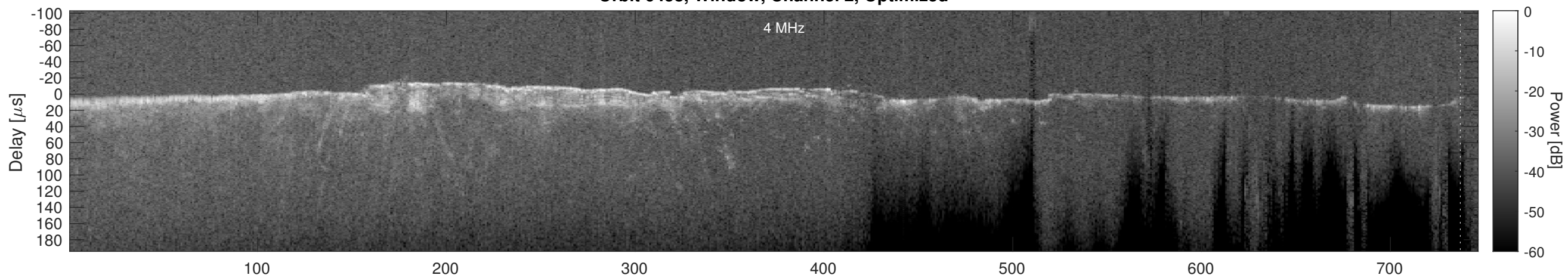
Orbit 6458, Cluttergram
