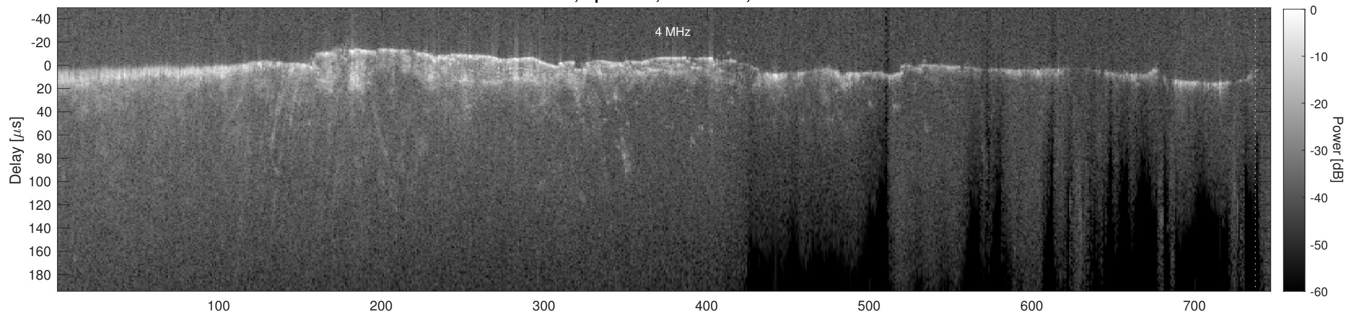
Orbit 6458, Cluttergram
