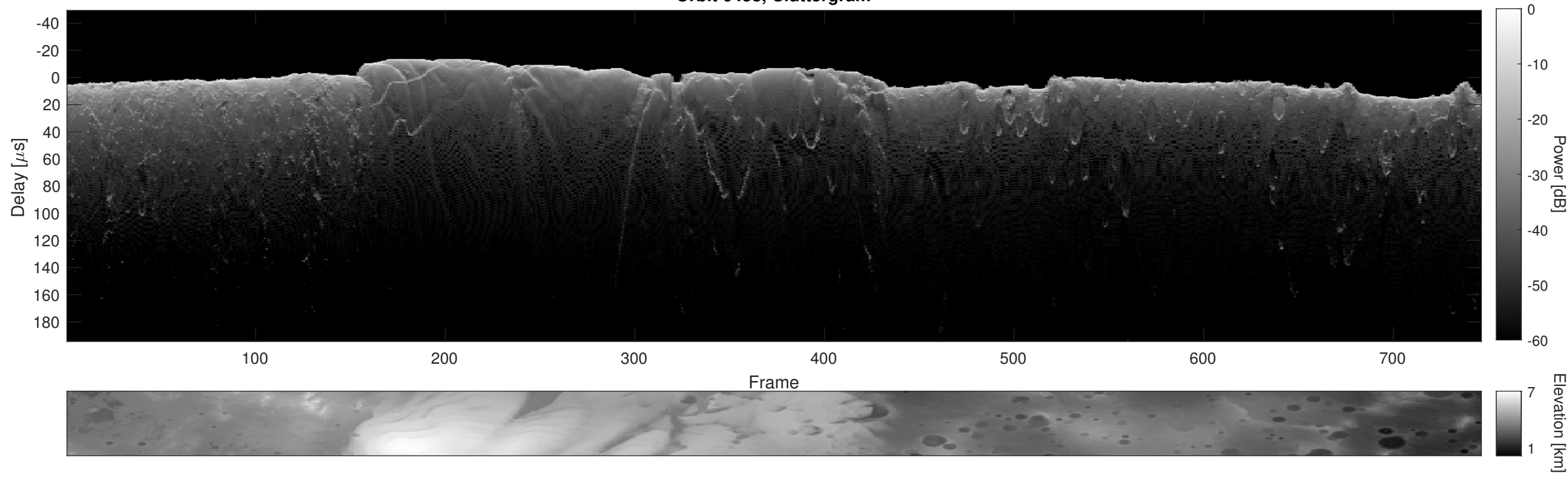
Orbit 6458, Cluttergram
