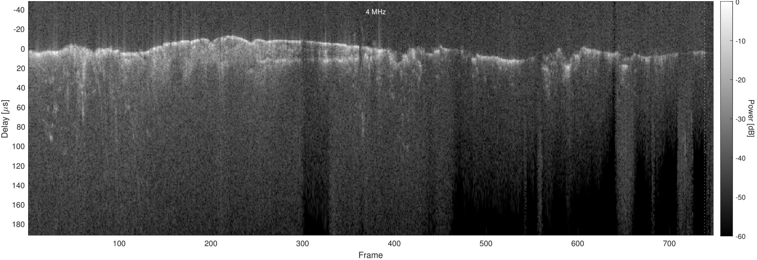
Orbit 6461, Optimized, No Window, Channel 2
