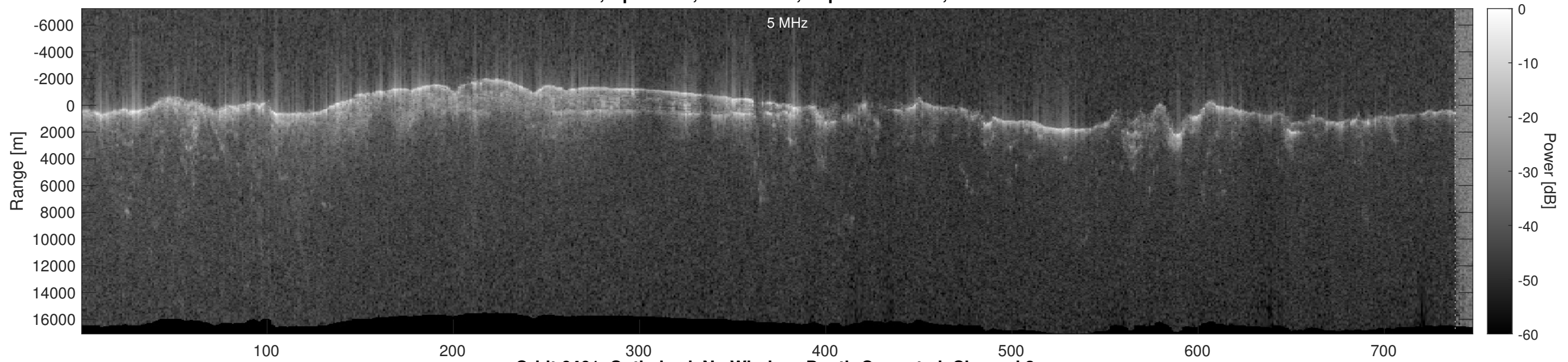
Orbit 6461, Optimized, No Window, Depth-Corrected, Channel 2
