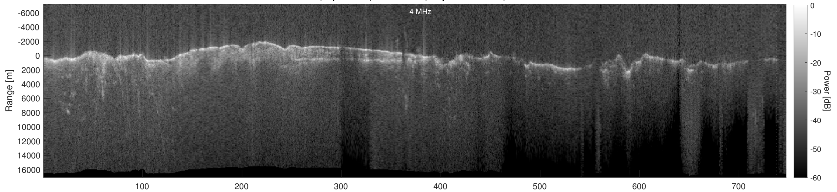
Orbit 6461, Depth-Corrected Cluttergram
