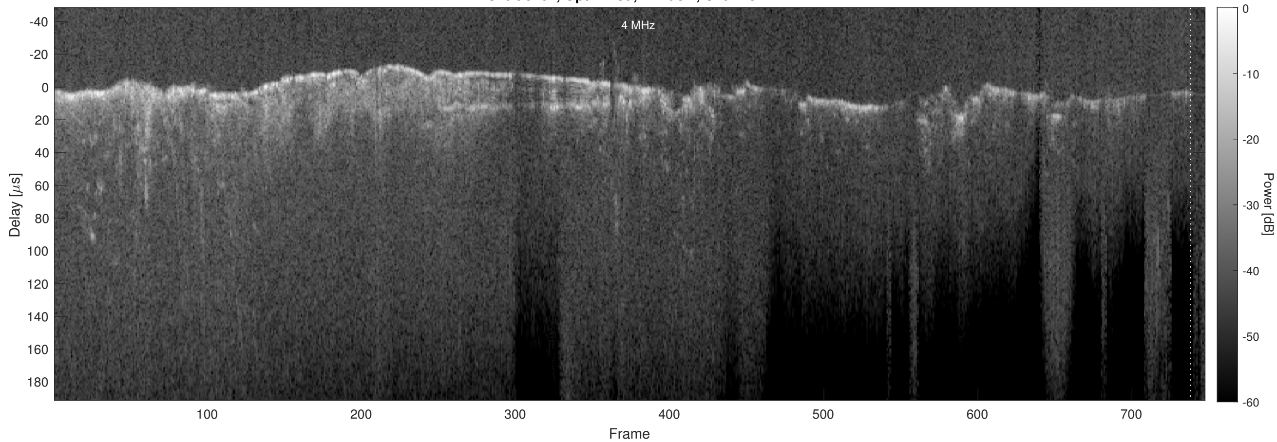
Orbit 6461, Optimized, Window, Channel 2
