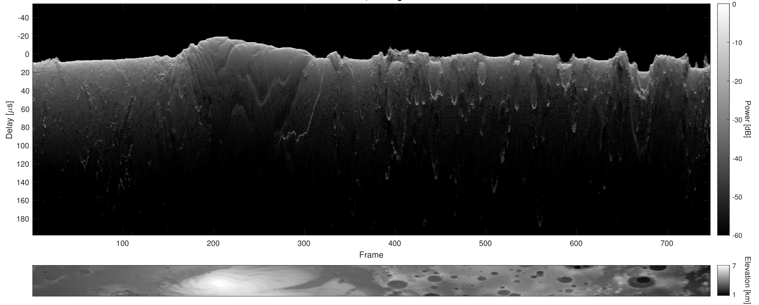
Orbit 6462, Cluttergram
