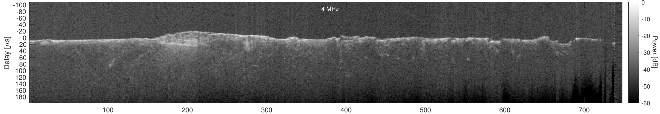
Orbit 6462, Cluttergram
