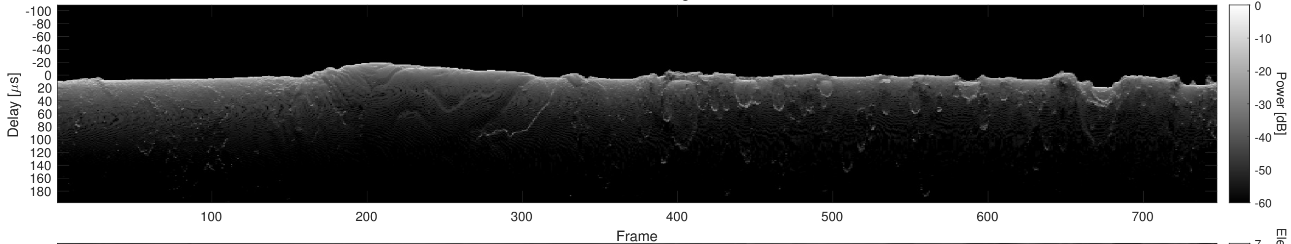
Orbit 6462, Cluttergram
