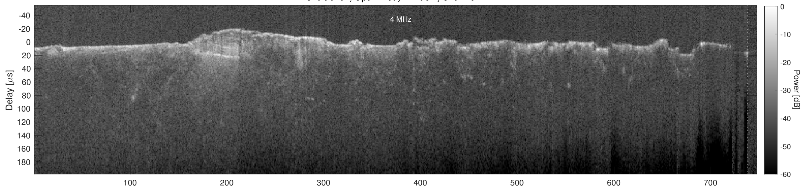
Orbit 6462, Cluttergram
