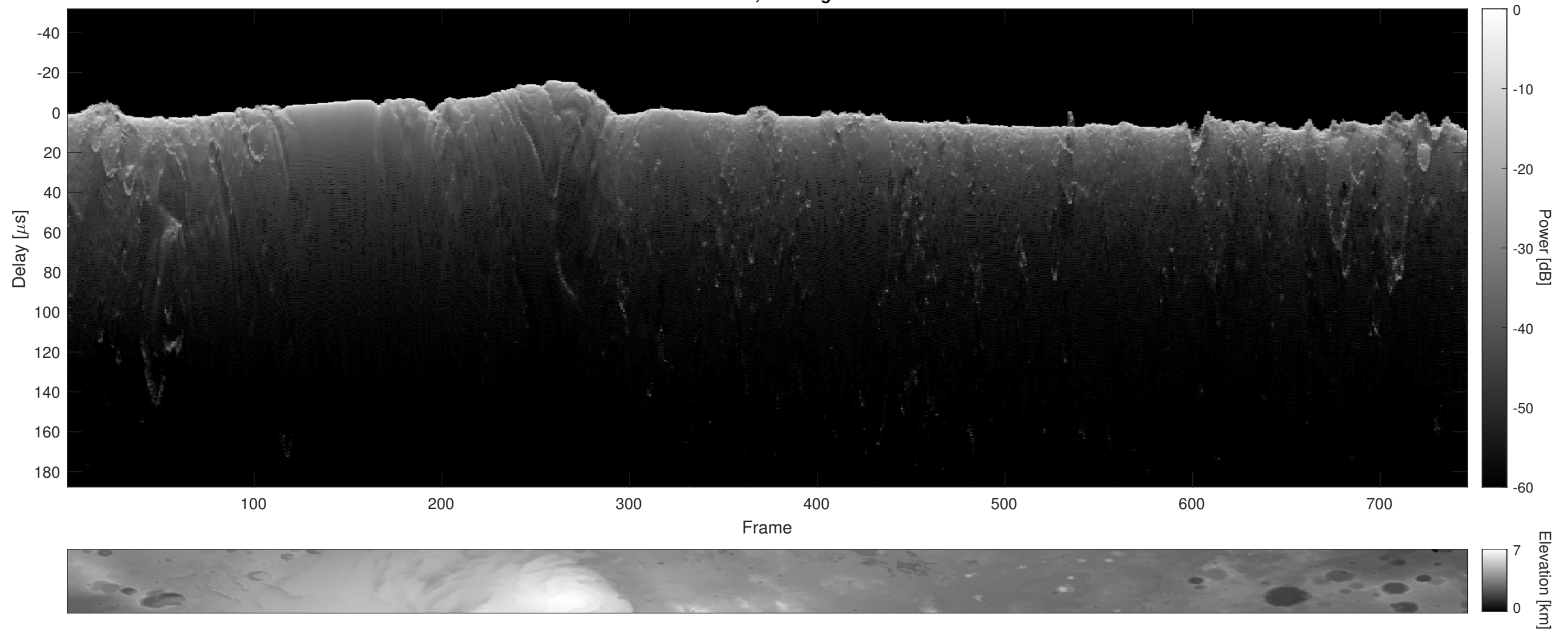
Orbit 6463, Cluttergram
