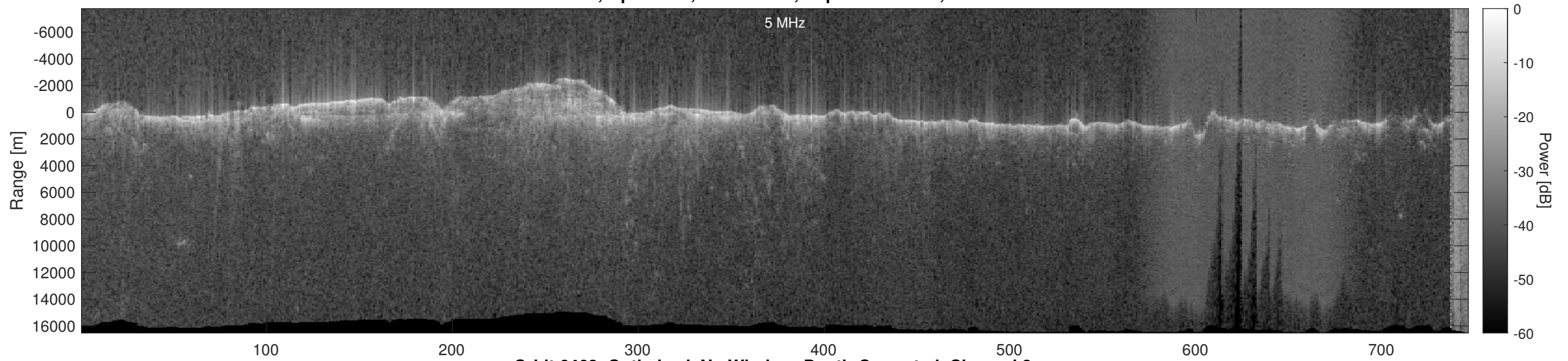
Orbit 6463, Optimized, No Window, Depth-Corrected, Channel 2
