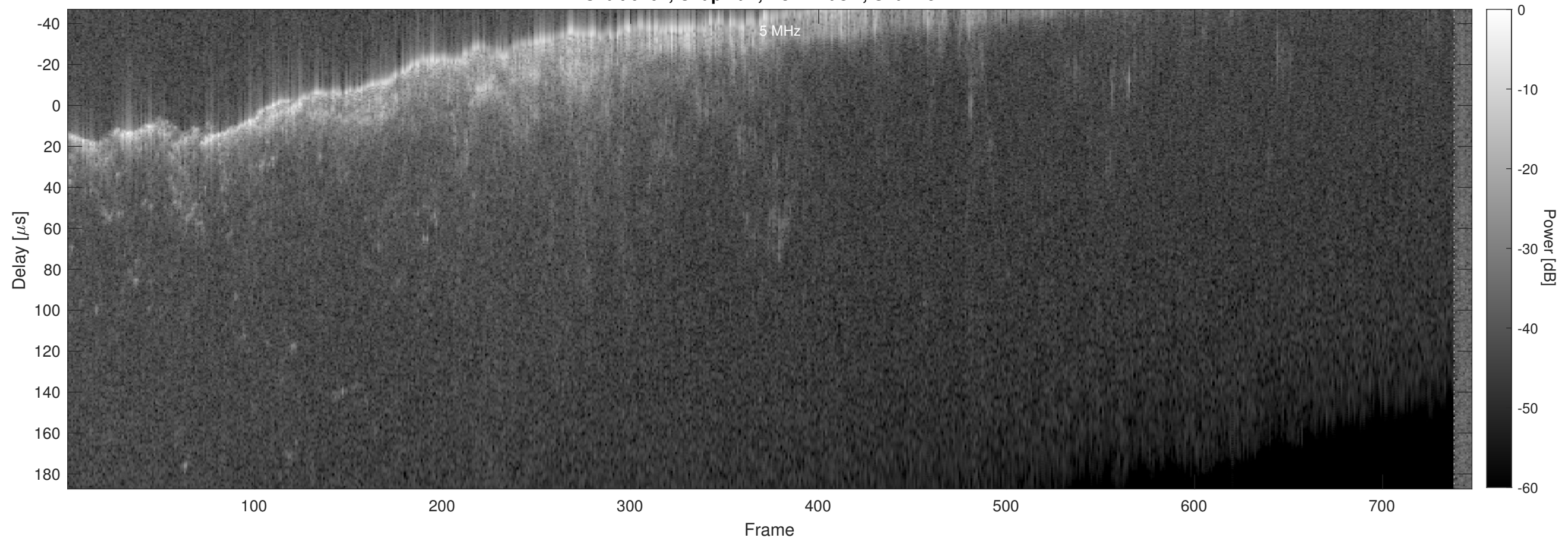
Orbit 6464, Chapman, No Window, Channel 2
