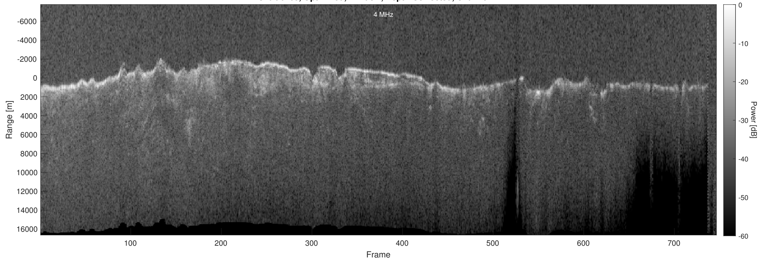
Orbit 6465, Optimized, Window, Depth-Corrected, Channel 2
