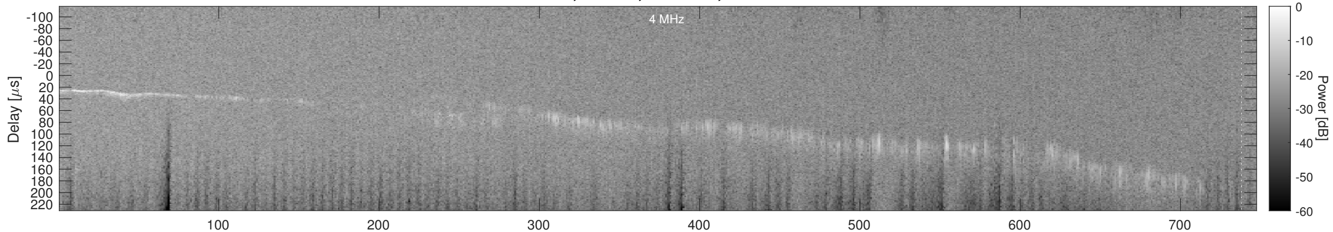
Orbit 6466, Window, Channel 2, Chapman
