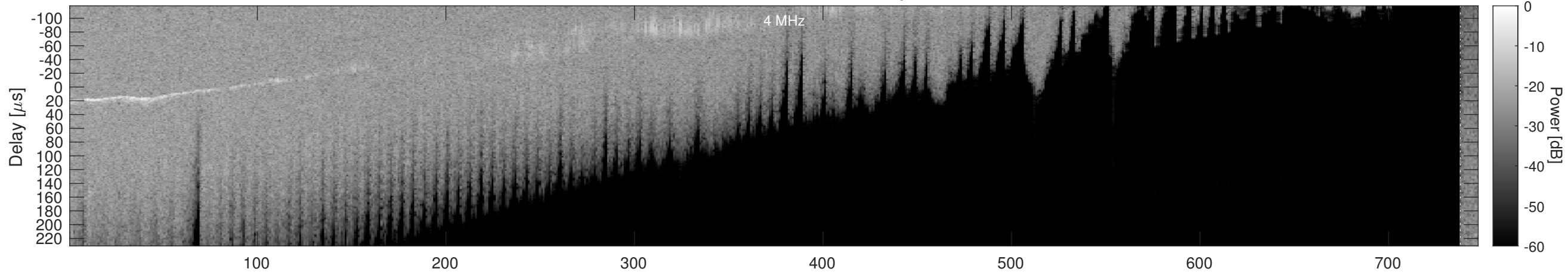
Orbit 6466, Window, Channel 2, Optimized
