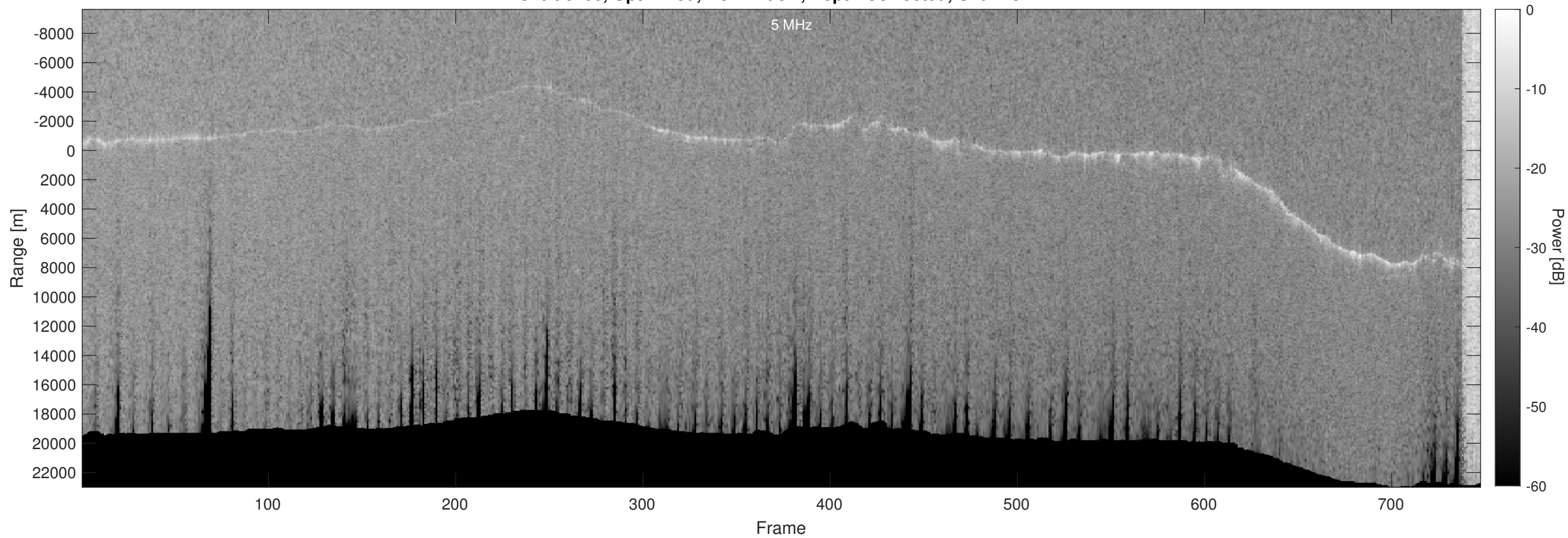
Orbit 6466, Optimized, No Window, Depth-Corrected, Channel 2
