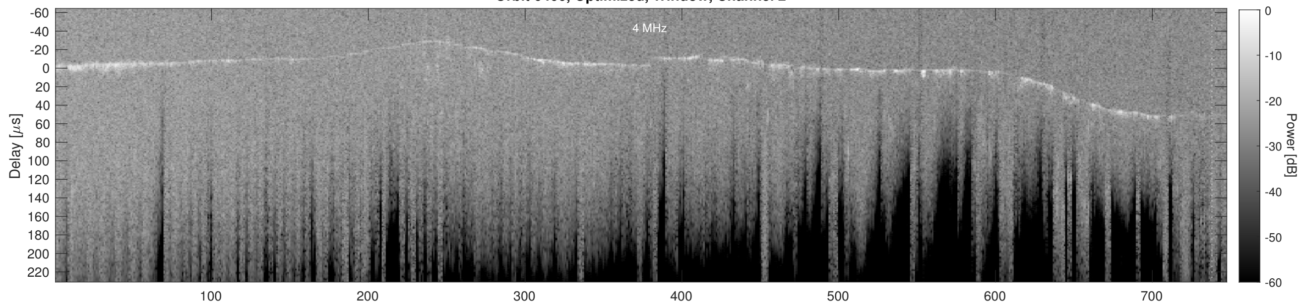
Orbit 6466, Cluttergram
