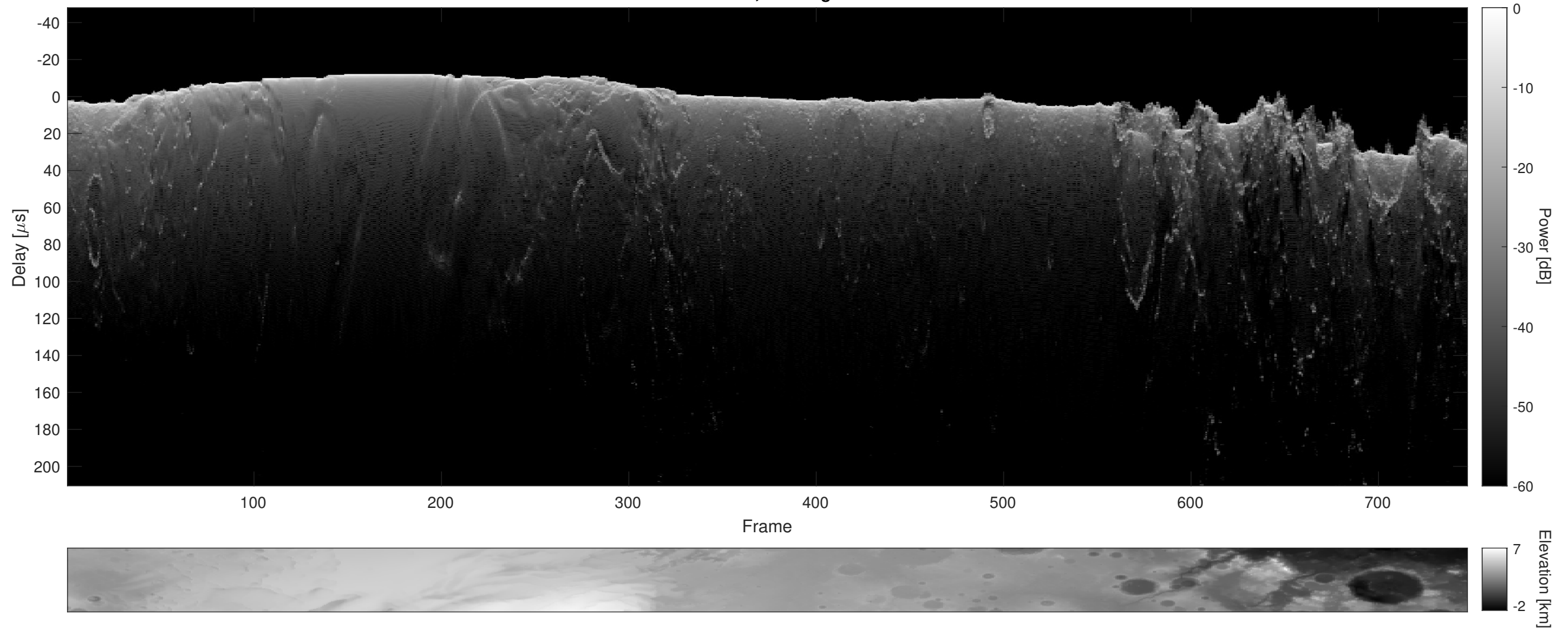
Orbit 6467, Cluttergram
