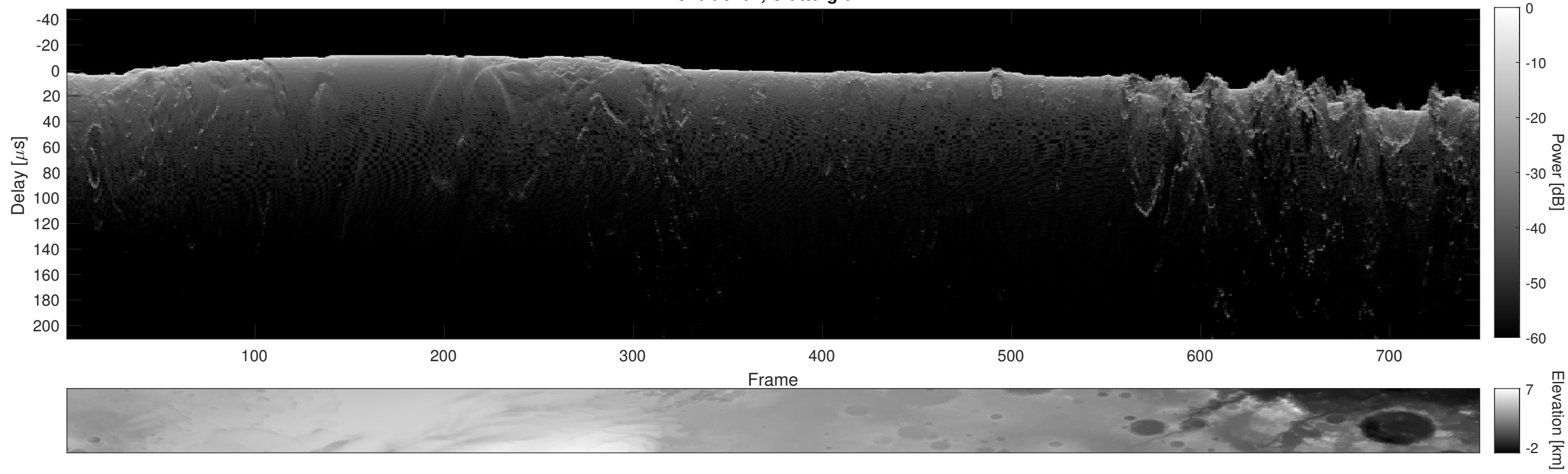
Orbit 6467, Cluttergram
