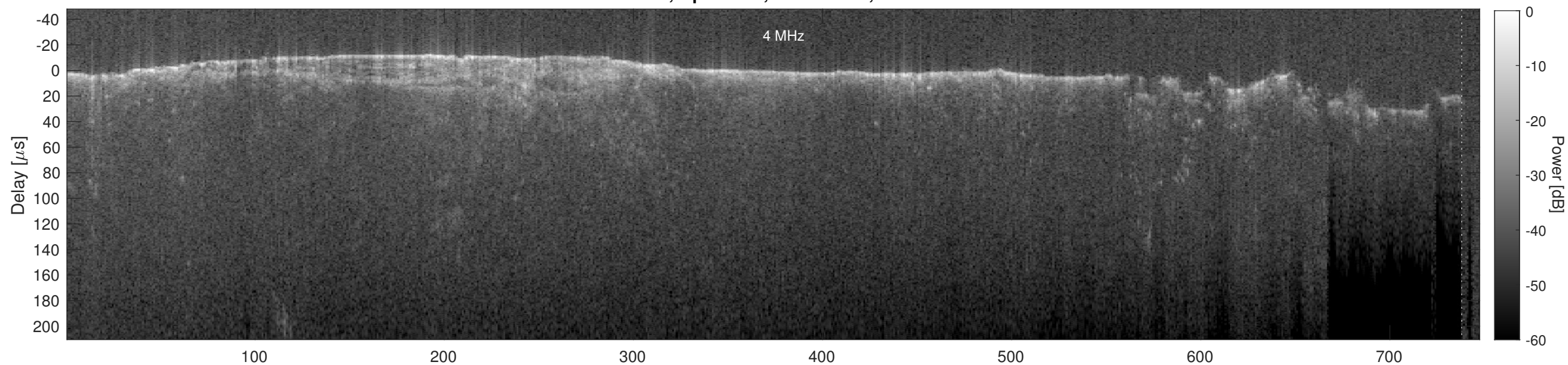
Orbit 6467, Cluttergram
