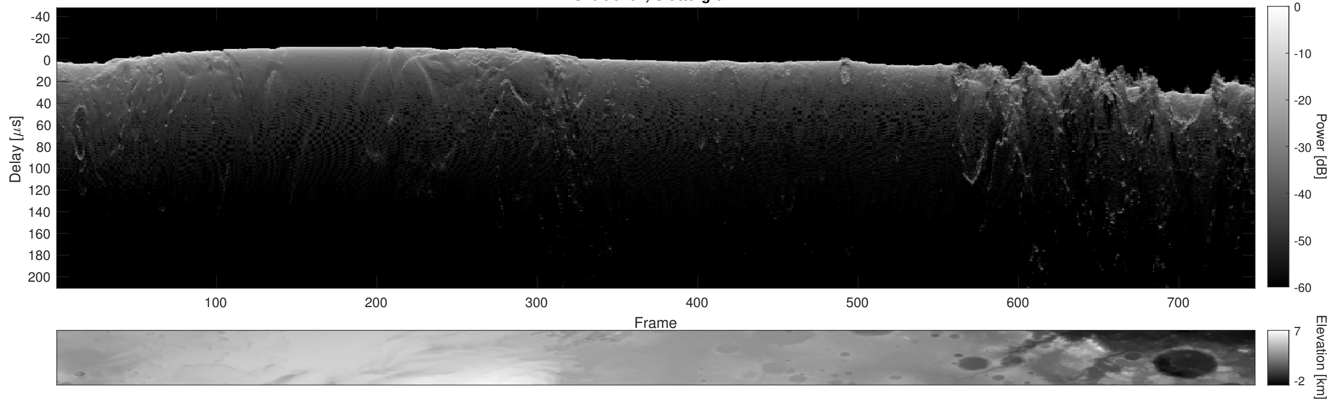
Orbit 6467, Cluttergram
