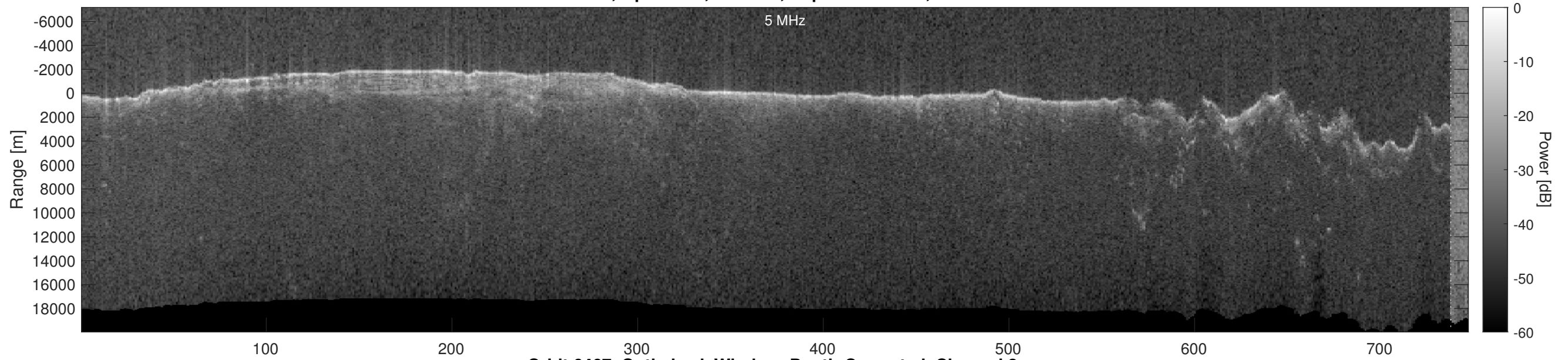
Orbit 6467, Optimized, Window, Depth-Corrected, Channel 2
