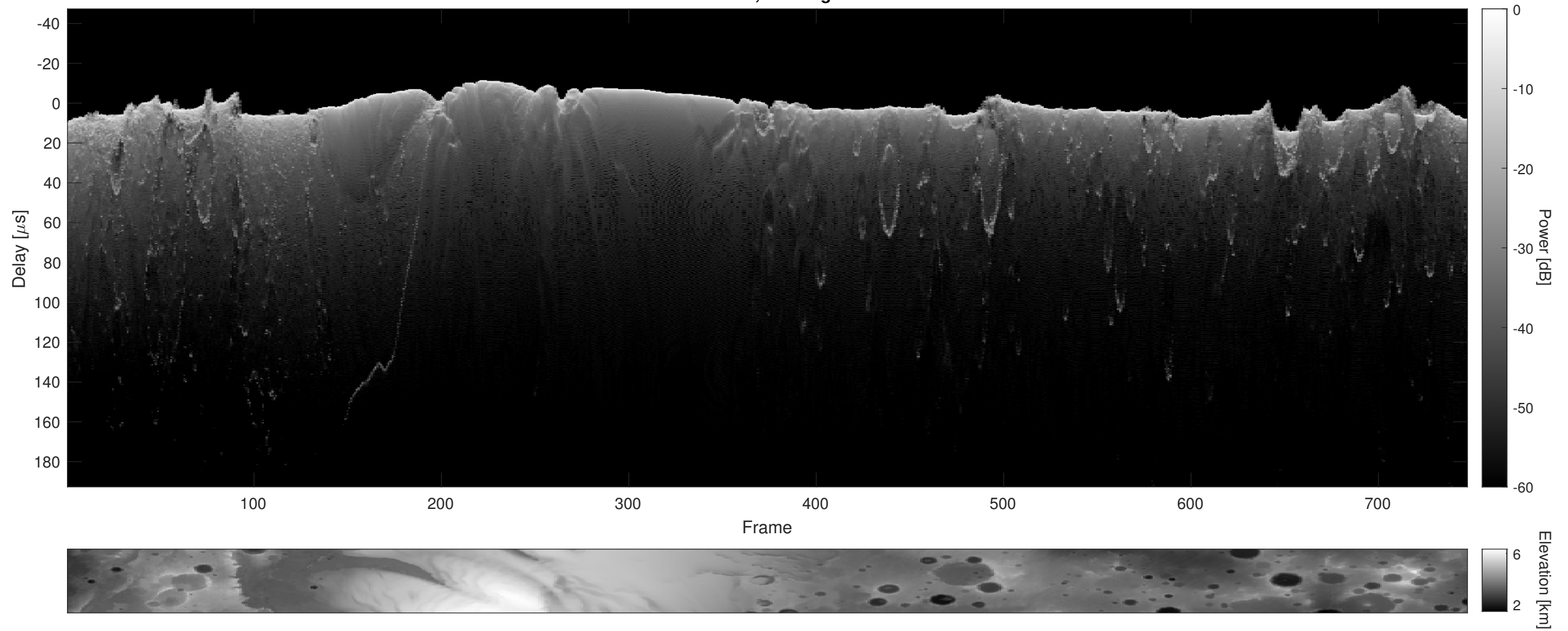
Orbit 6468, Cluttergram
