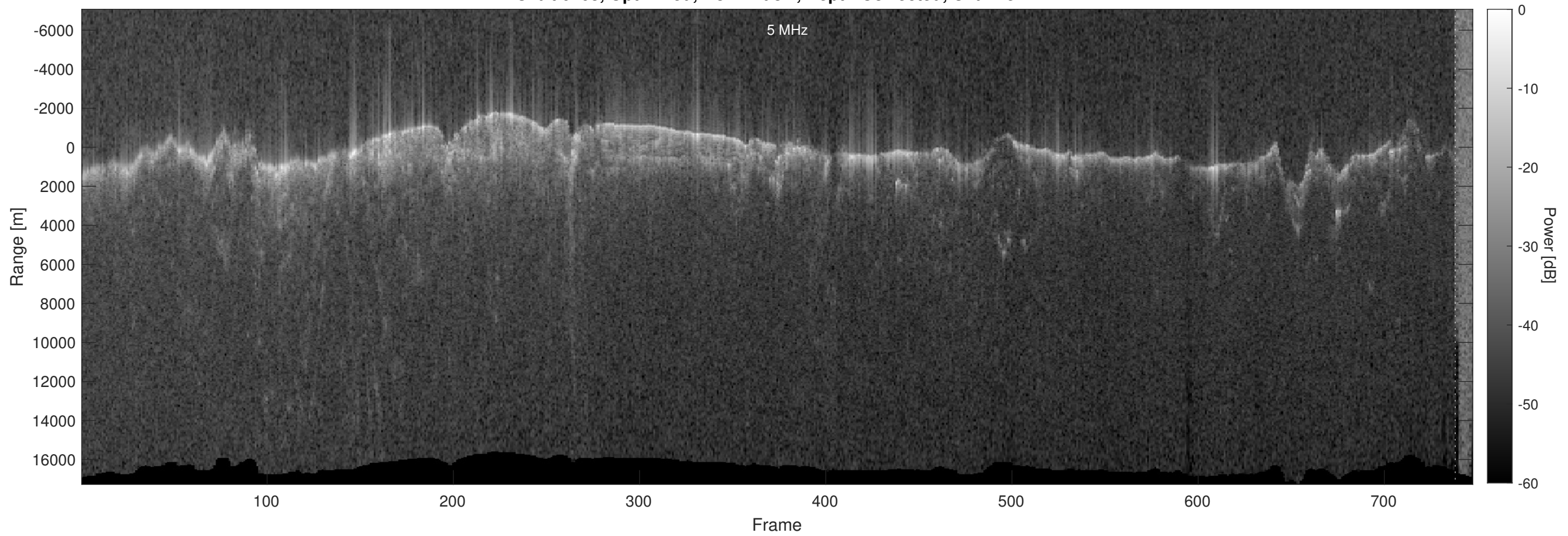
Orbit 6468, Optimized, No Window, Depth-Corrected, Channel 2
