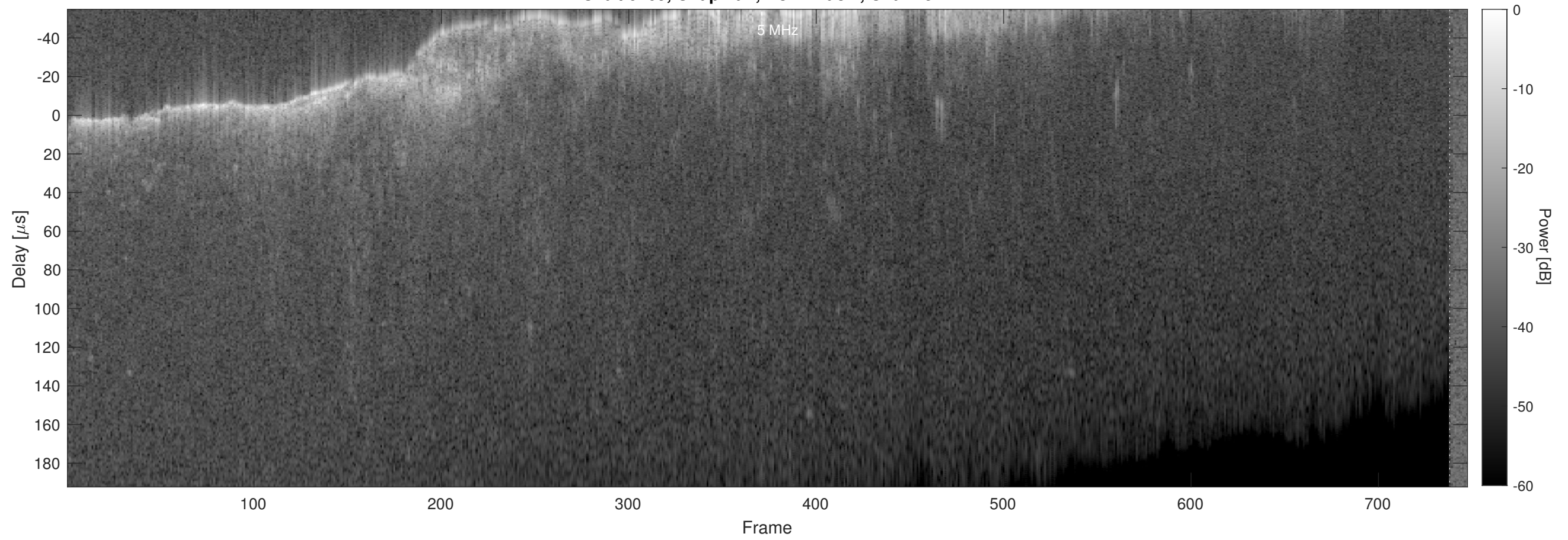
Orbit 6469, Chapman, No Window, Channel 2
