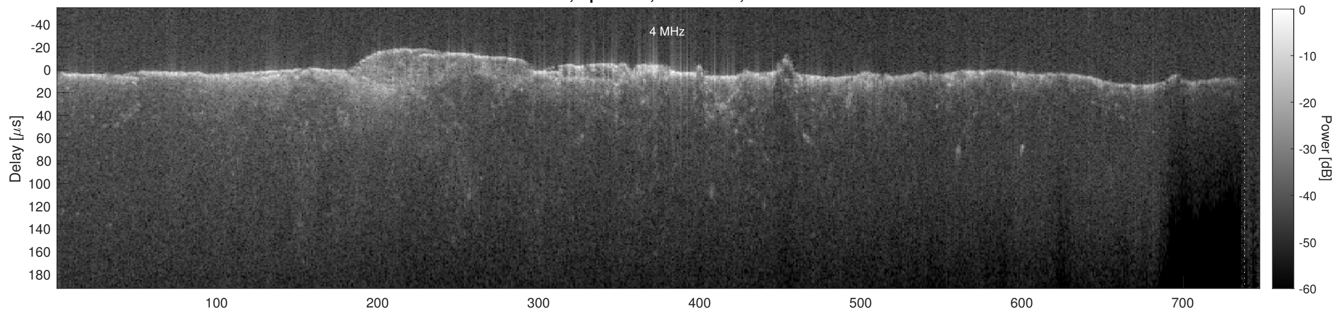
Orbit 6469, Cluttergram
