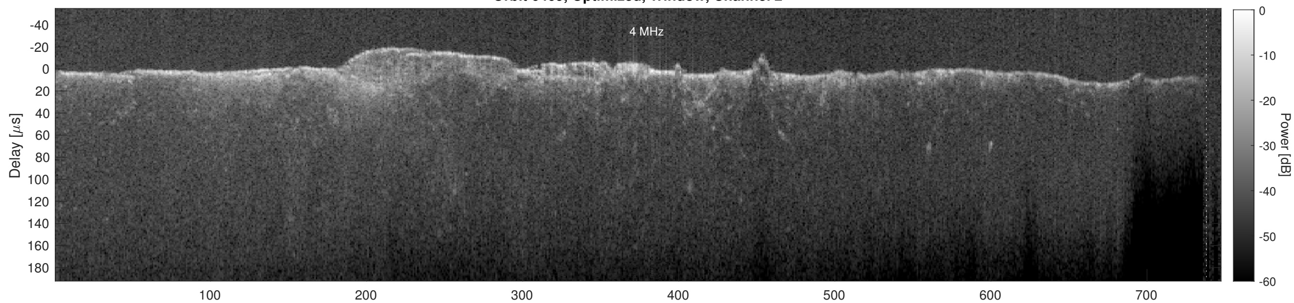
Orbit 6469, Cluttergram
