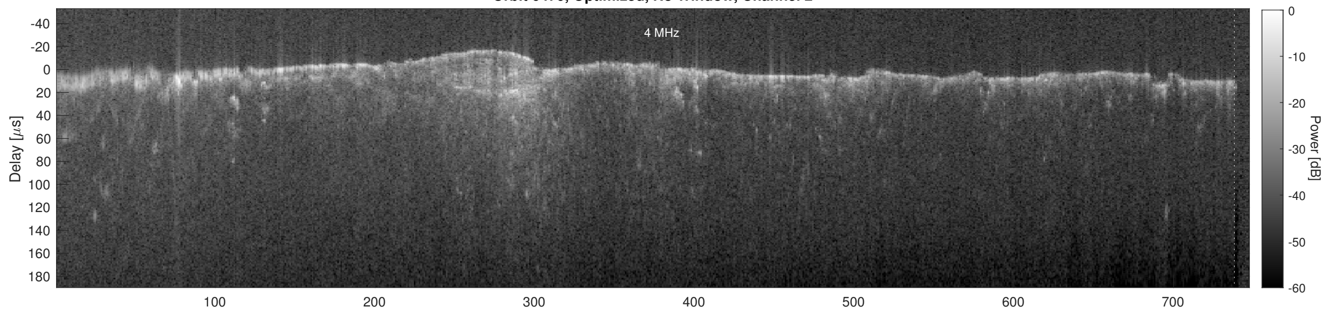
Orbit 6470, Cluttergram
