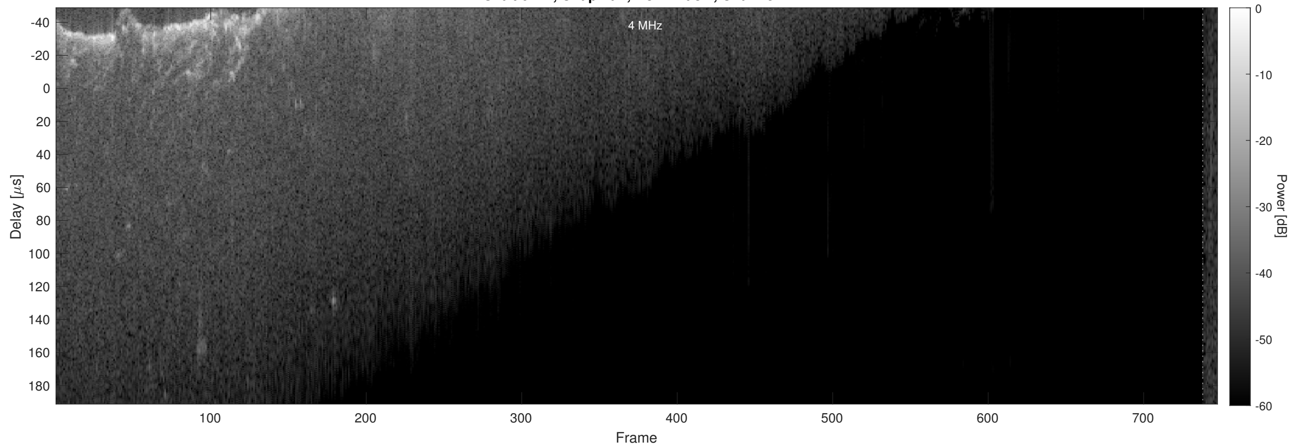
Orbit 6471, Chapman, No Window, Channel 2
