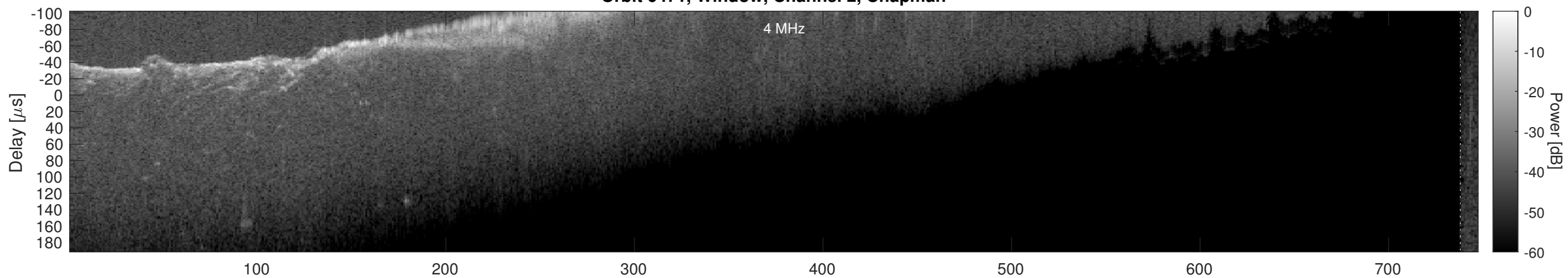
Orbit 6471, Window, Channel 2, Optimized
