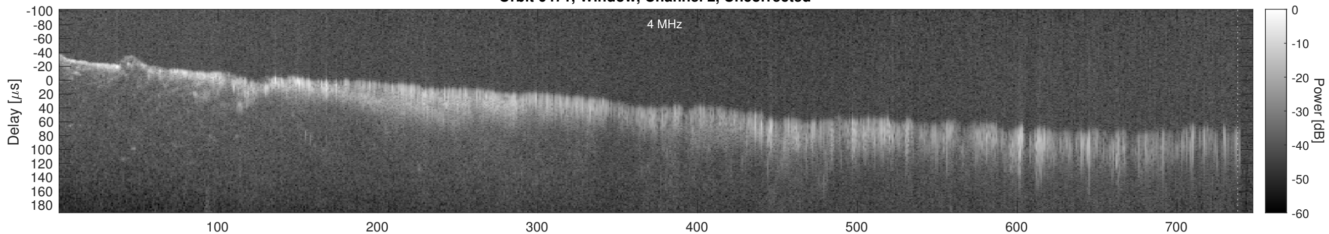
Orbit 6471, Window, Channel 2, Chapman
