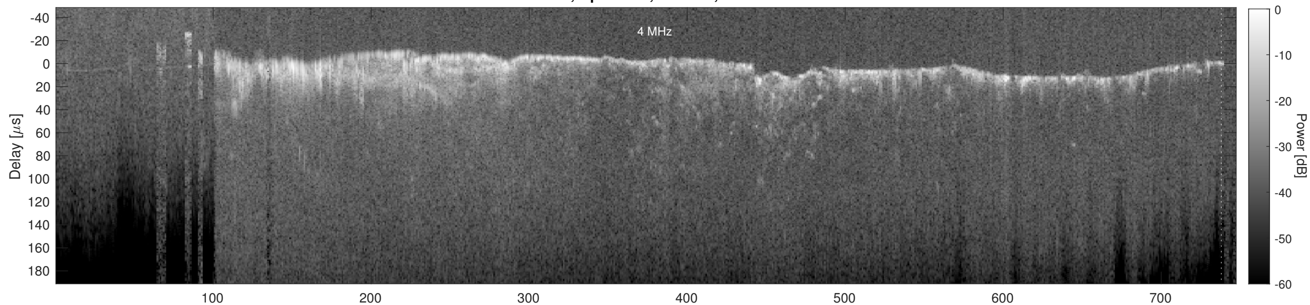
Orbit 6471, Cluttergram
