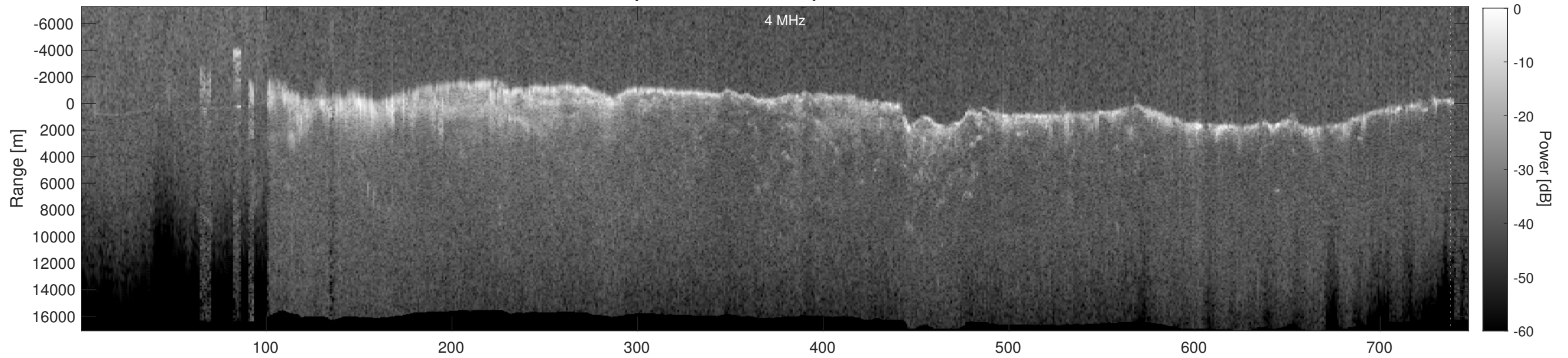
Orbit 6471, Depth-Corrected Cluttergram
