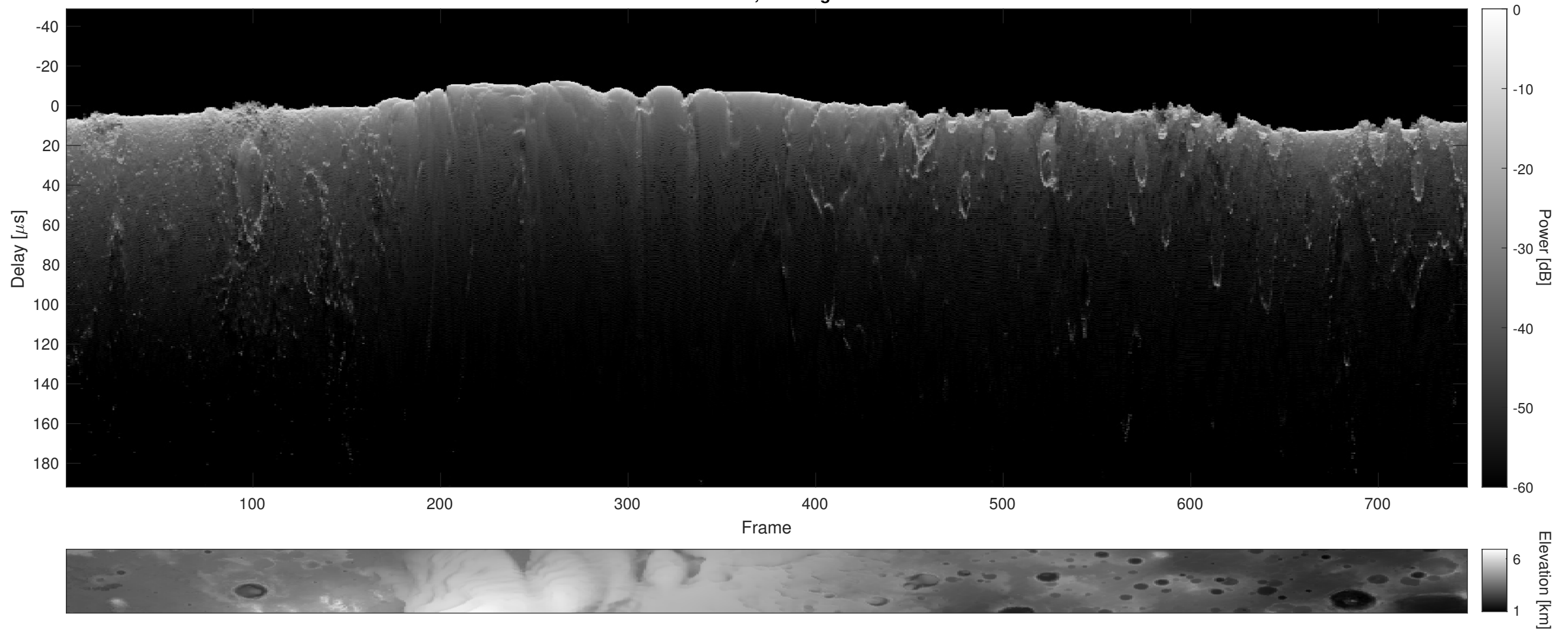
Orbit 6472, Cluttergram
