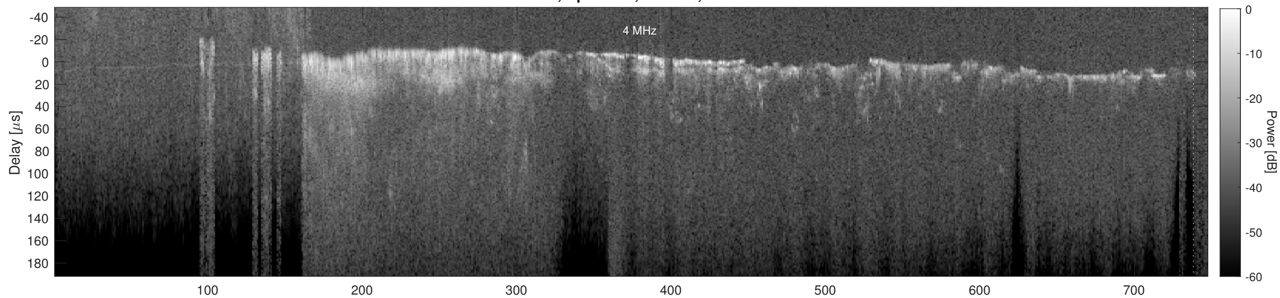
Orbit 6472, Cluttergram
