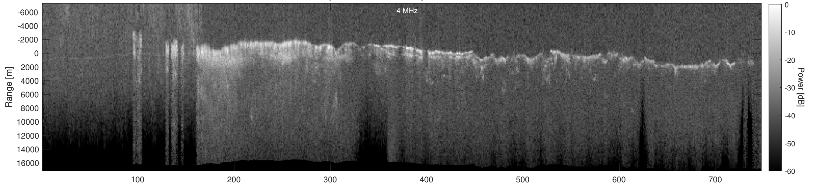
Orbit 6472, Depth-Corrected Cluttergram
