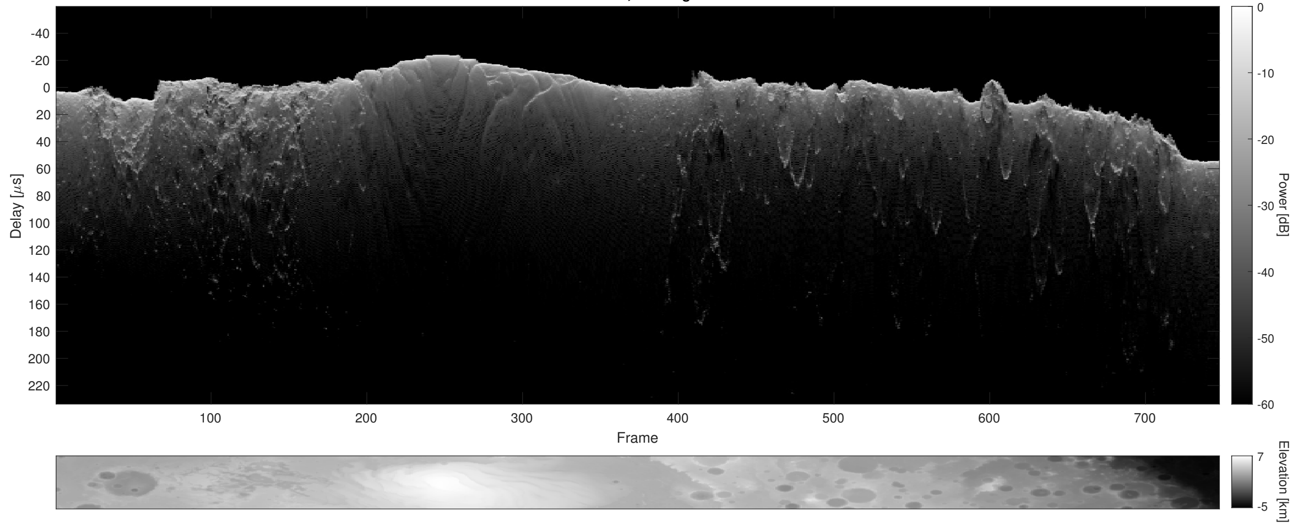
Orbit 6473, Cluttergram
