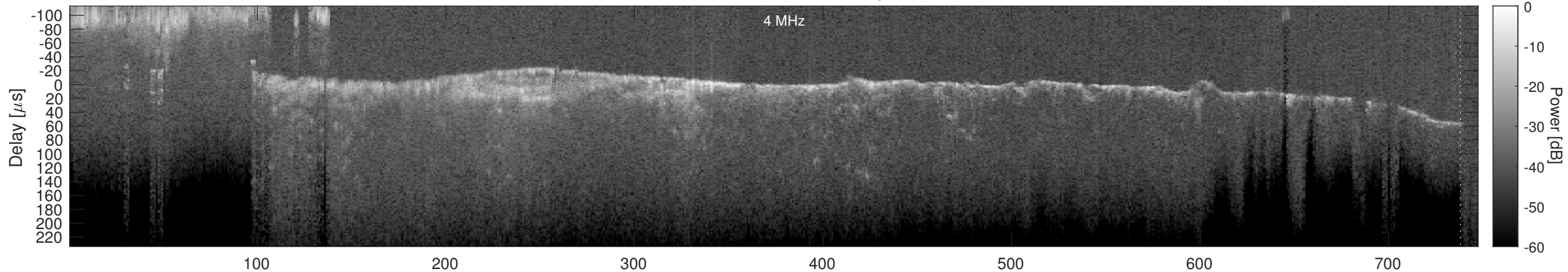
Orbit 6473, Cluttergram
