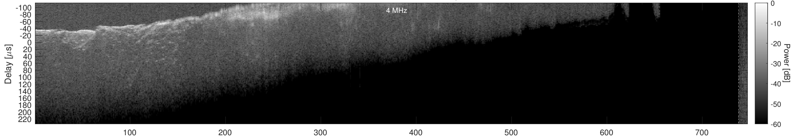
Orbit 6473, Window, Channel 2, Optimized
