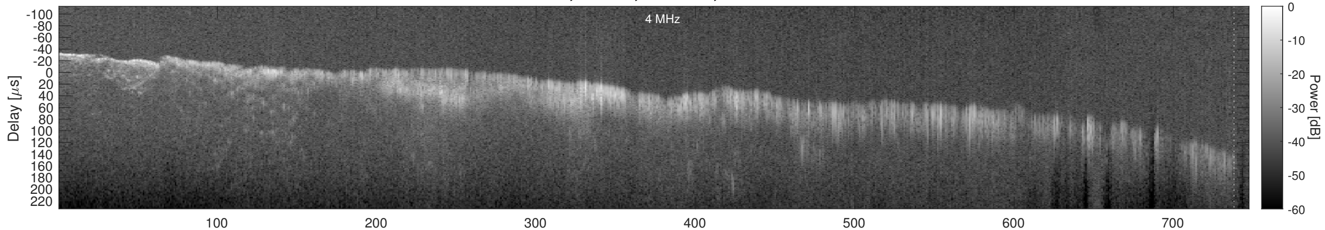
Orbit 6473, Window, Channel 2, Chapman
