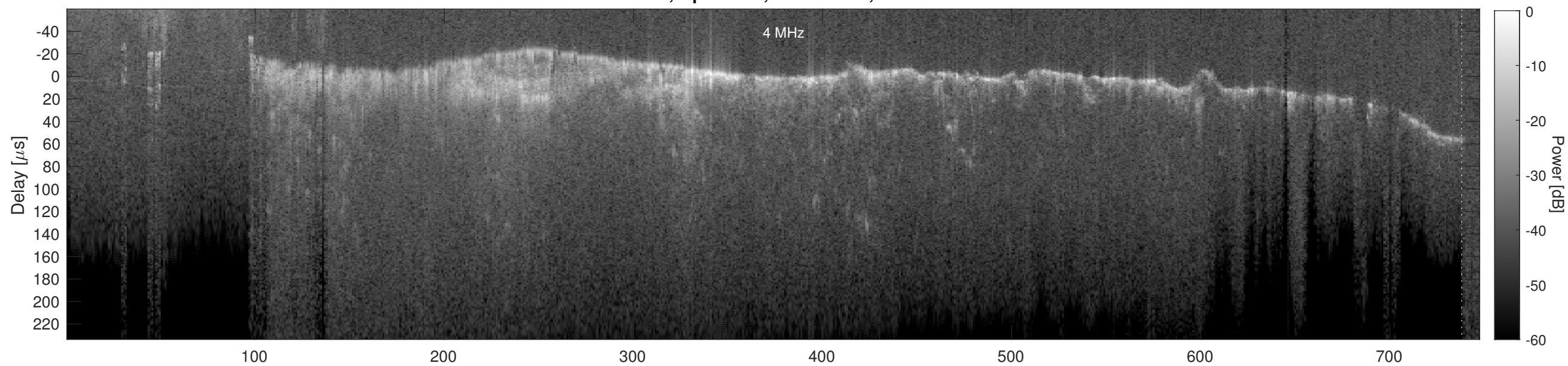
Orbit 6473, Cluttergram
