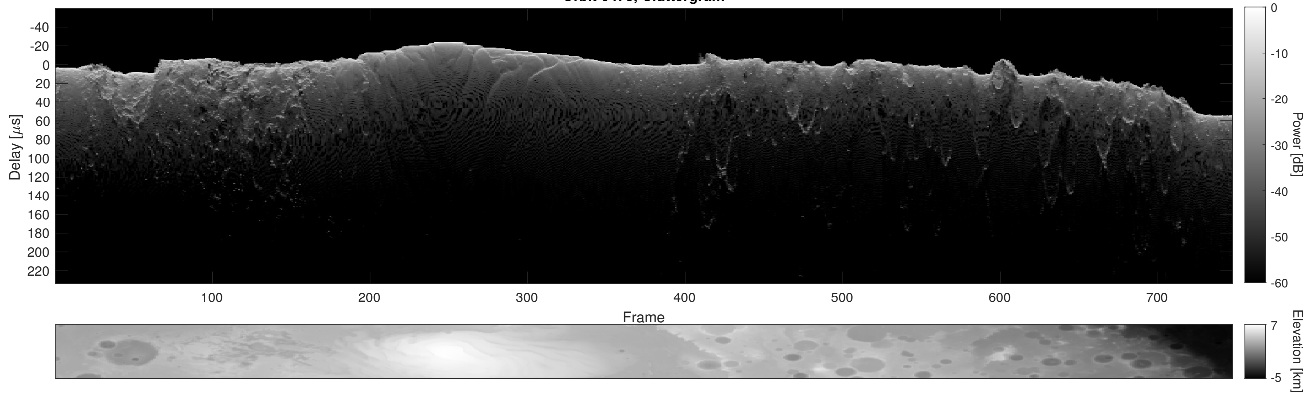
Orbit 6473, Cluttergram
