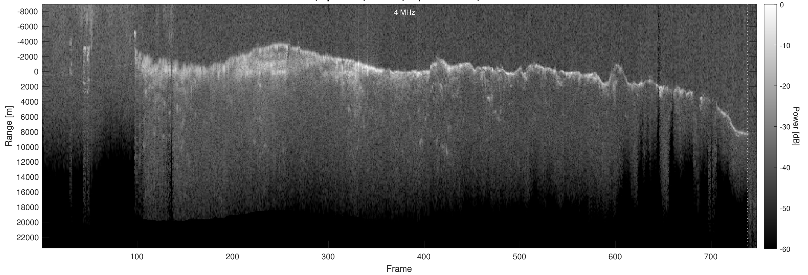
Orbit 6473, Optimized, Window, Depth-Corrected, Channel 2
