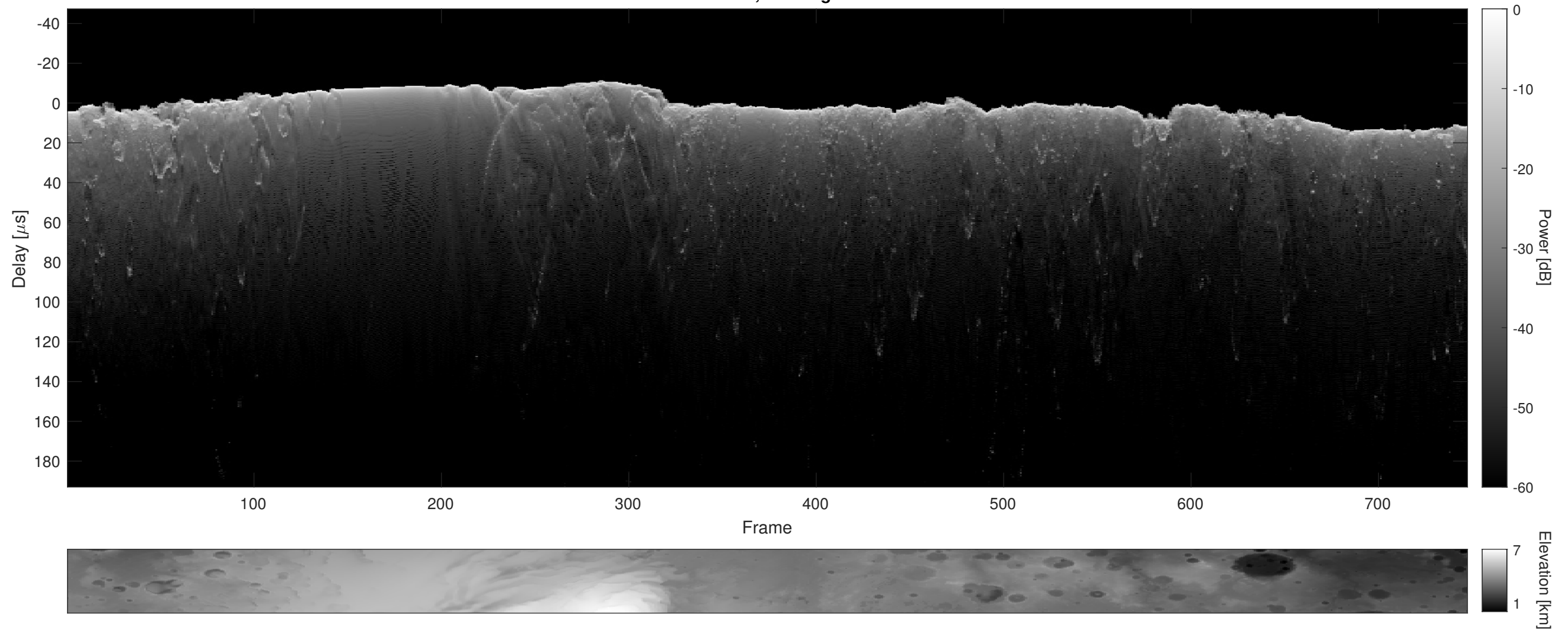
Orbit 6474, Cluttergram
