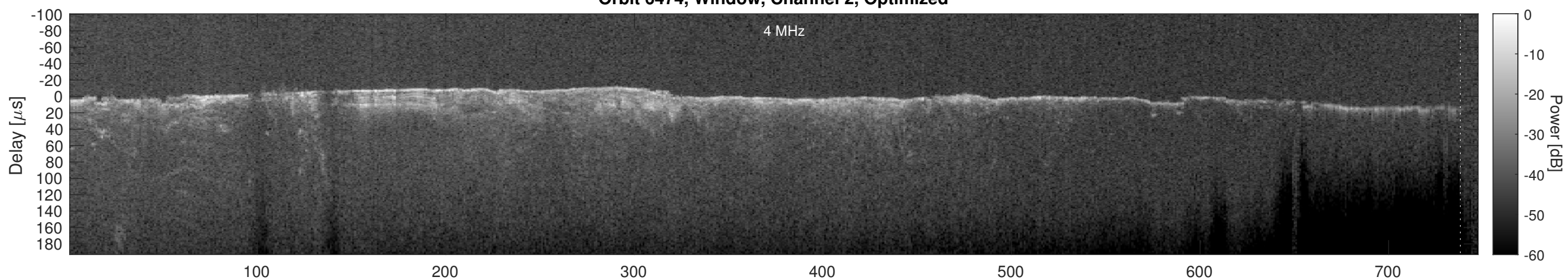
Orbit 6474, Cluttergram
