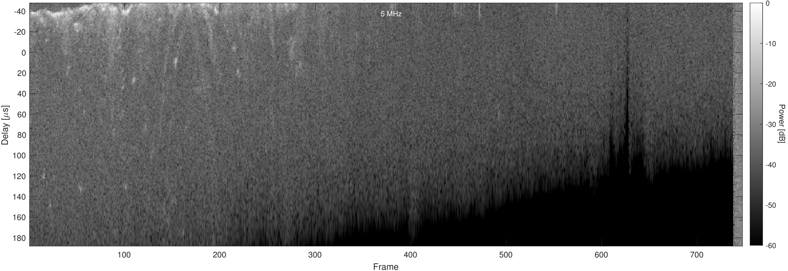
Orbit 6475, Chapman, Window, Channel 2
