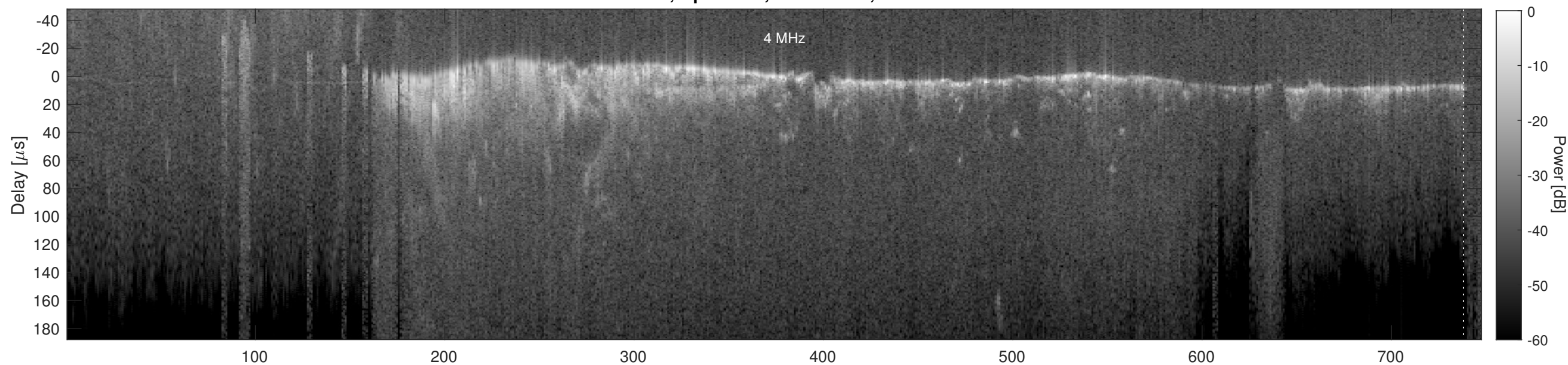
Orbit 6475, Cluttergram
